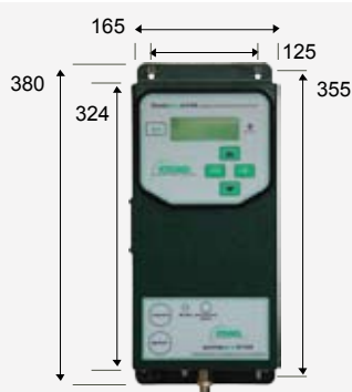
Dimensions in mm Depth = 90 (3.5")
