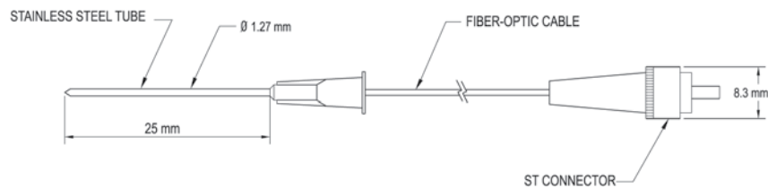
Model FOT-N
