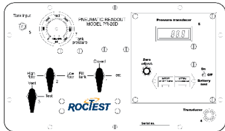
PR-20D Control Panel
