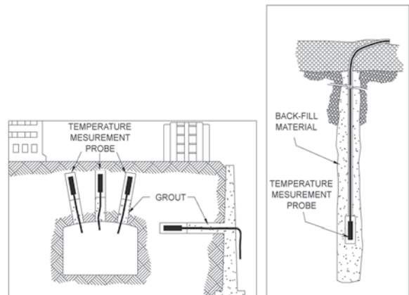
TH Probe Typical Installations
